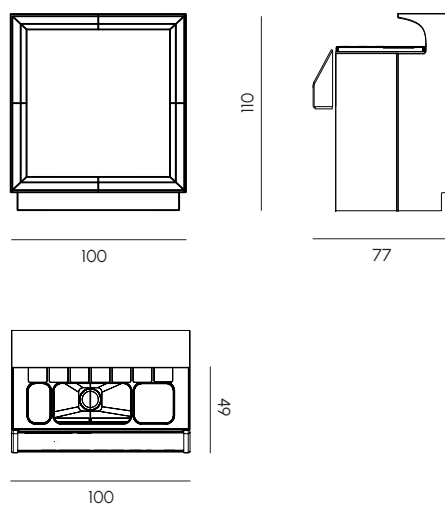
Dublin modulo lineare con cocktail station ABS Dublin straight element with ABS cocktail station
