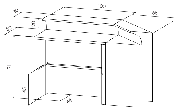
Misure tridimensionali del bancone Counter three-dimensional measures
