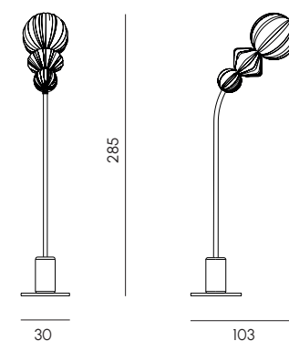
Joy lampada da terra con base in marmo Joy standing lamp with marble base
